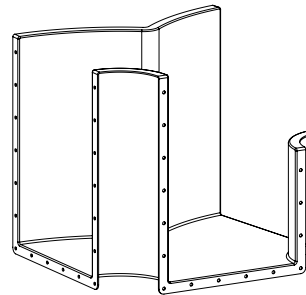
4 - Floor element (side view)
