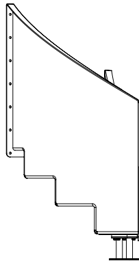
2 - Step up element (side view)
