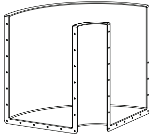
3 - Step off (side view)
